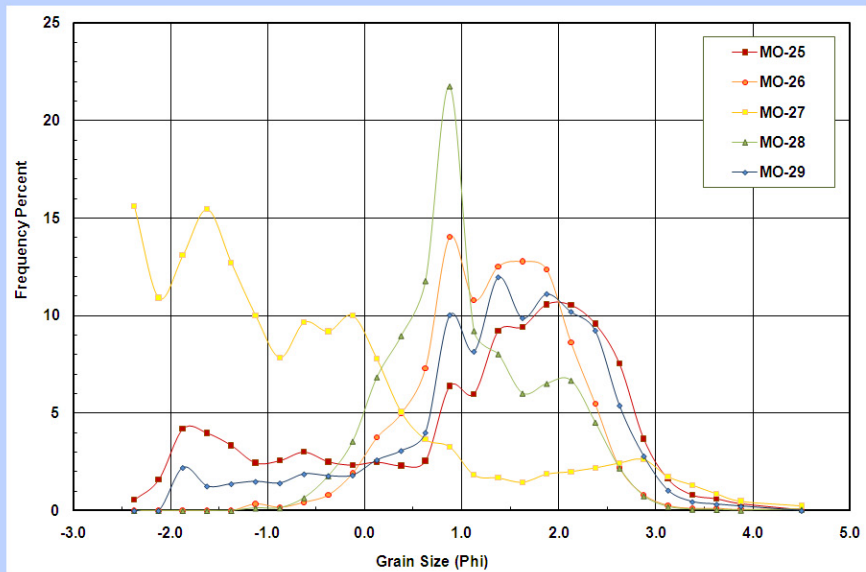
Figure 14 - Grain Size Distribution Comparisons of the Lower Keys
