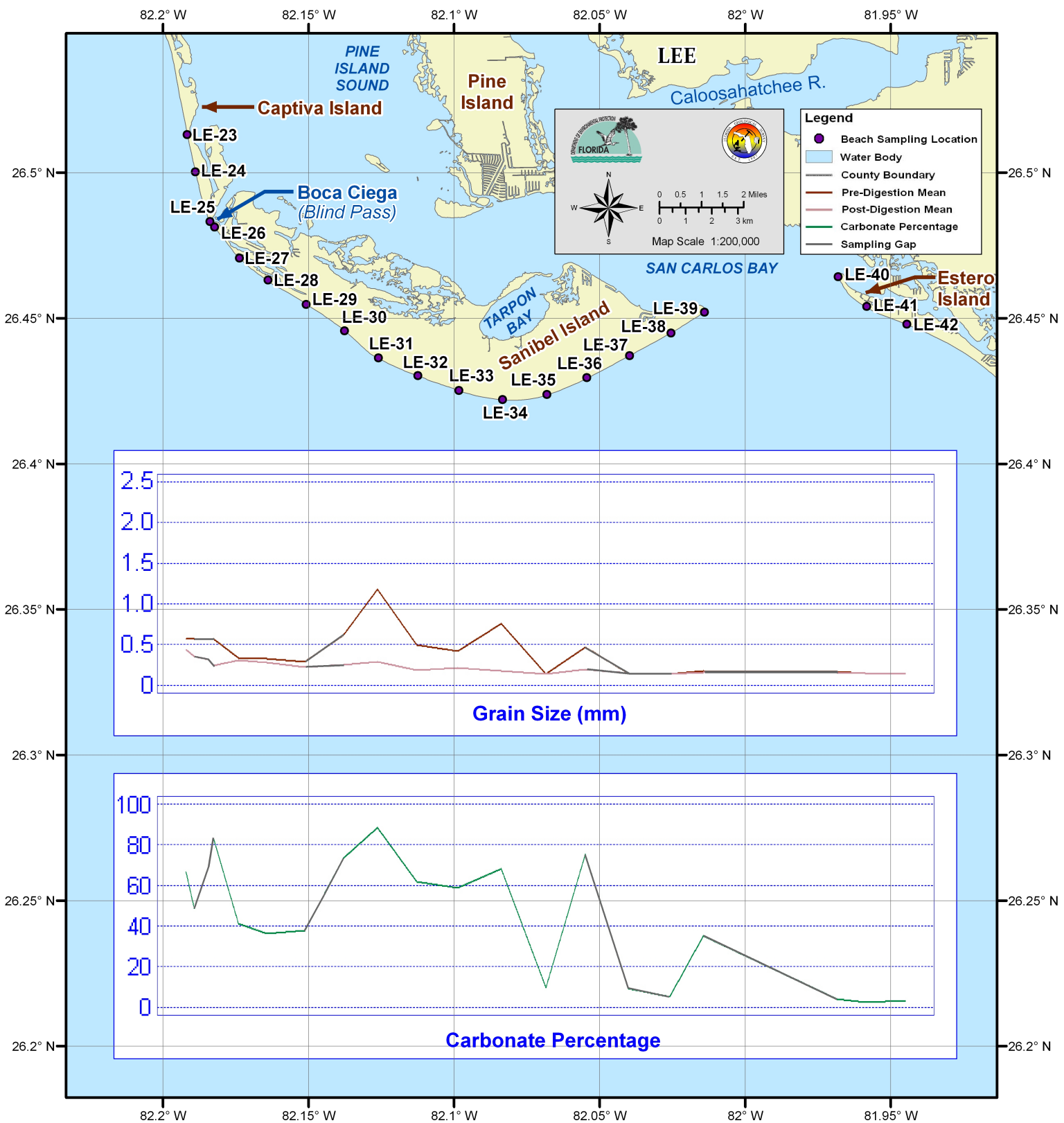
Figure 11: Grain Size and Carbonate Percentage from Boca Ciega to San Carlos Bay (Sanibel Island)
