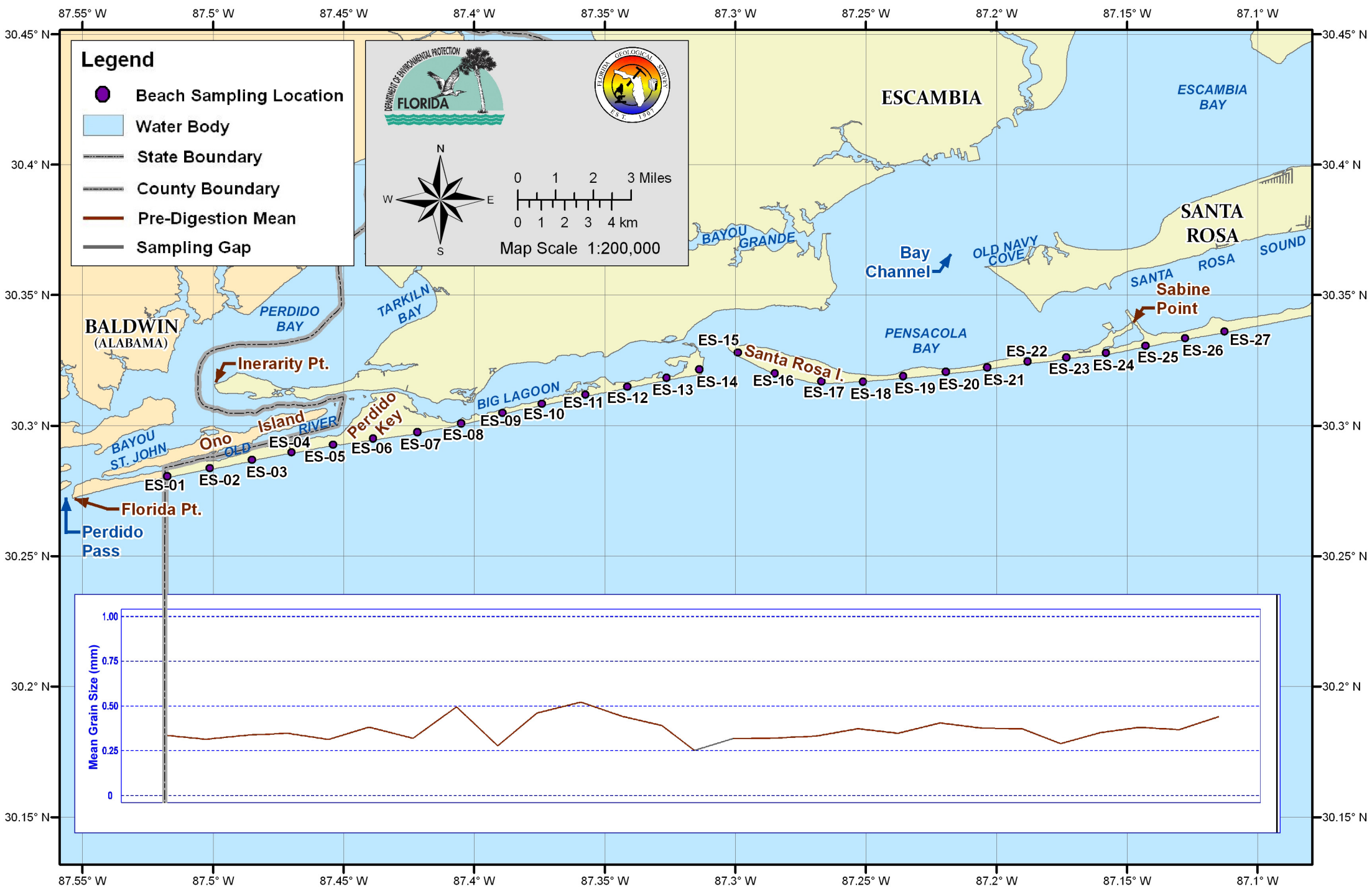
Figure 9. Mean grain size from the Alabama-Florida state line to Sabine Point
