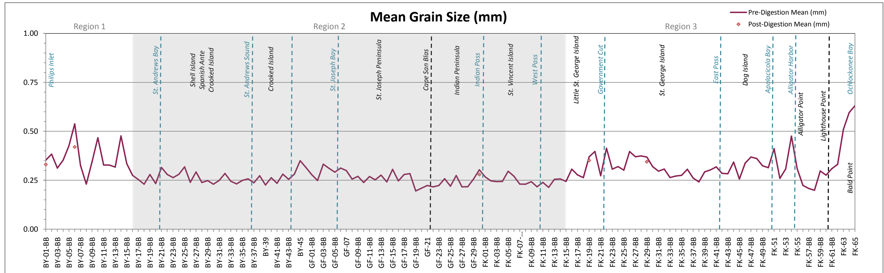
Figure 21 - Mean Grain Size over the beaches of the northwest coast of Florida
