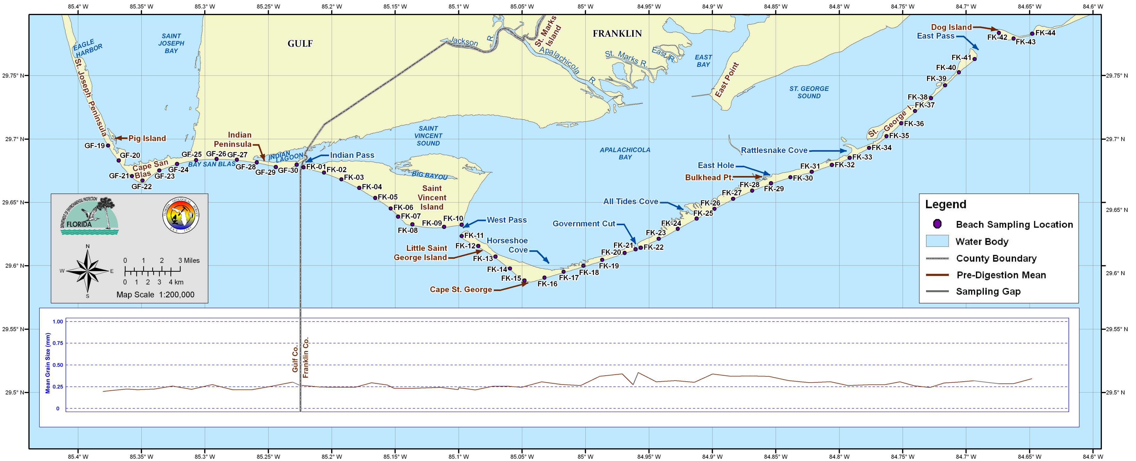
Figure 14. Mean grain size from Cape San Blas to East Pass
