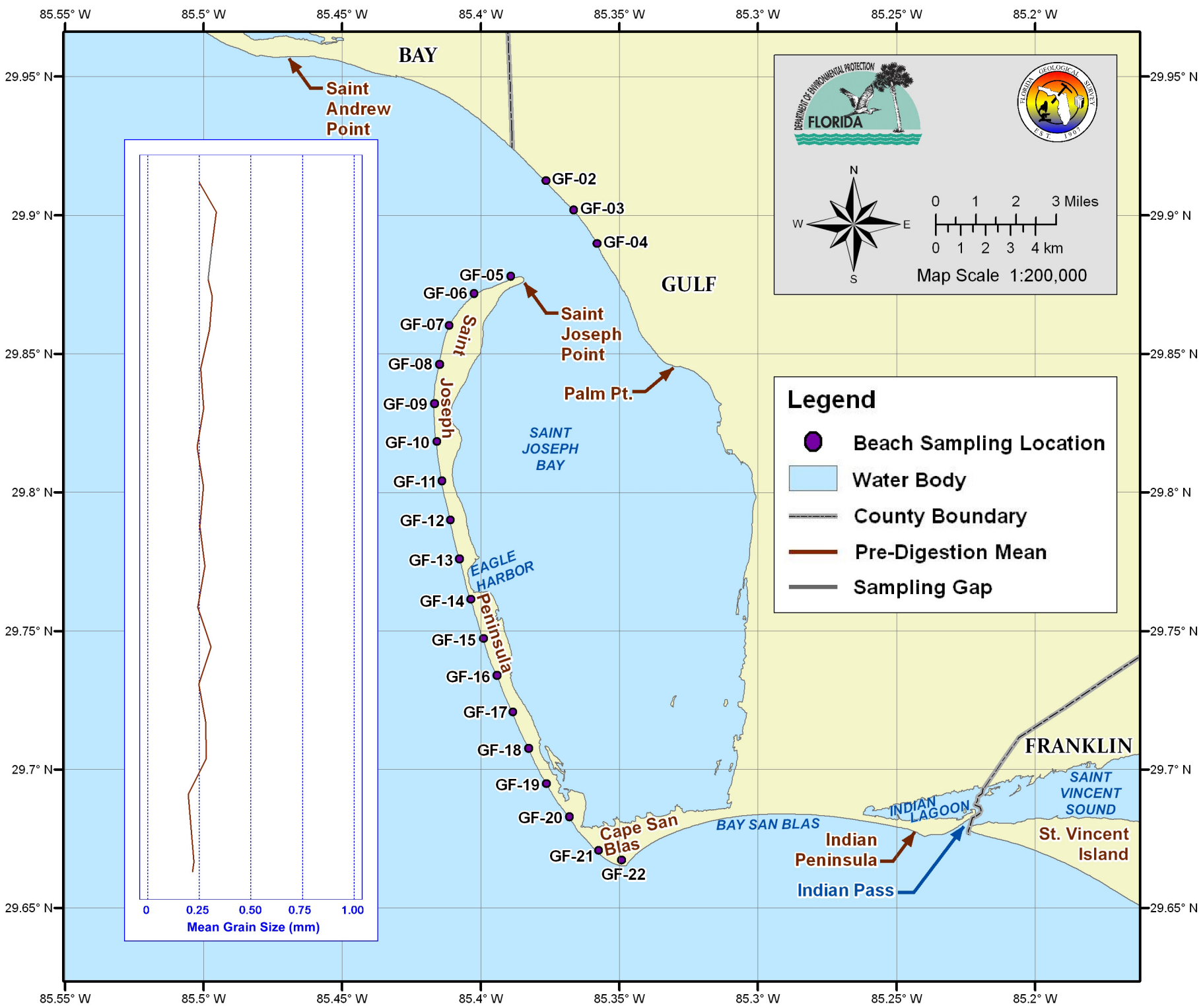
Figure 13. Mean grain size from St. Joseph Point to Cape San Blas
